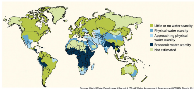
FIGURE 2 Global Physical and Economic Water Scarcity
