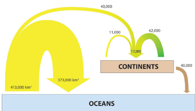
Global Terrestrial Water Cycle
